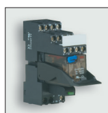
DC relay, 4 changeover contacts / 4PDT, pluggable, AgNi, AgNi +5 μm HV Page 61
