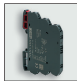
Output relay, 1 changeover contact / SPDT, AgSnO 2 , + 5 μm HV Page 33
